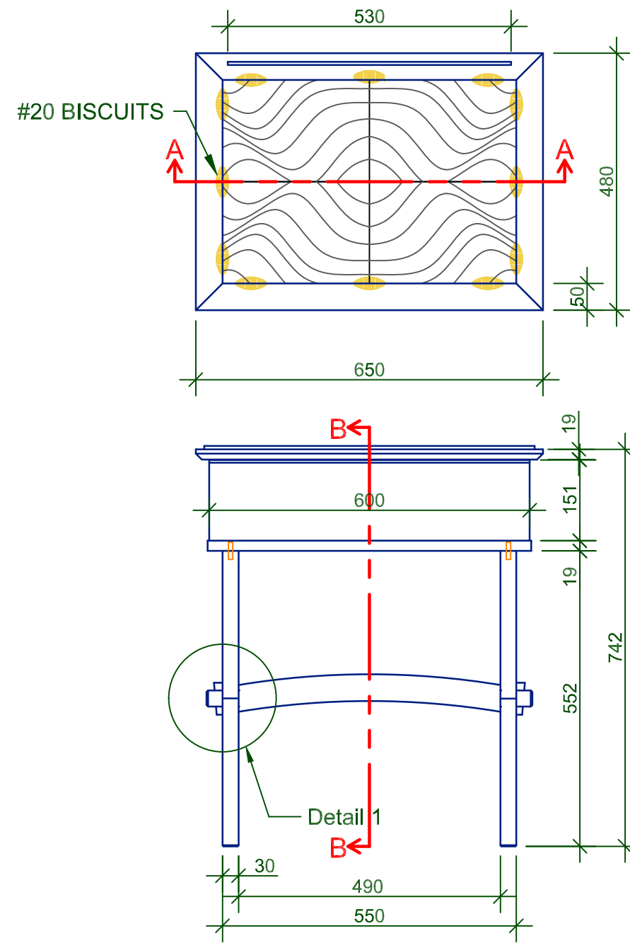
Orthographic Views
