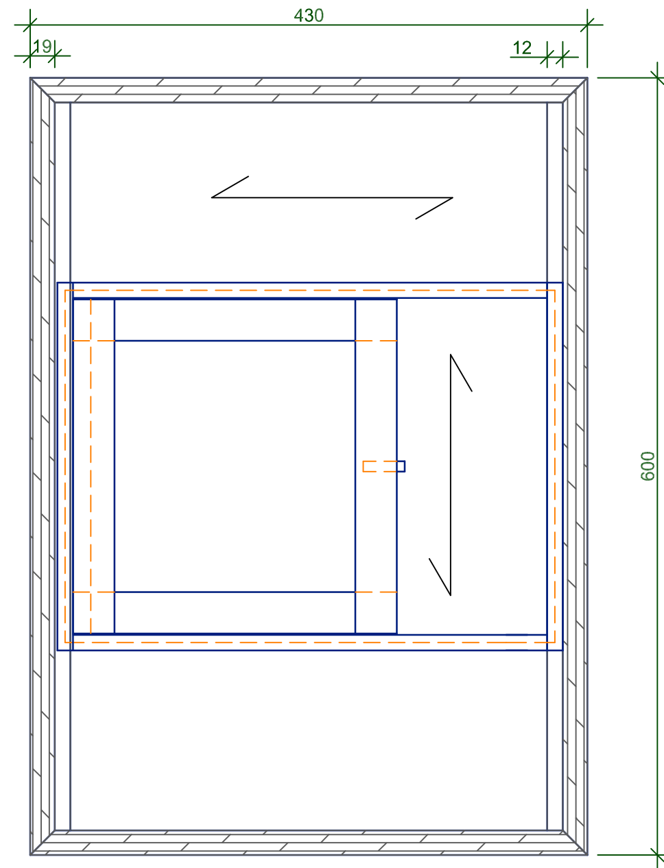
SECTION C-C
