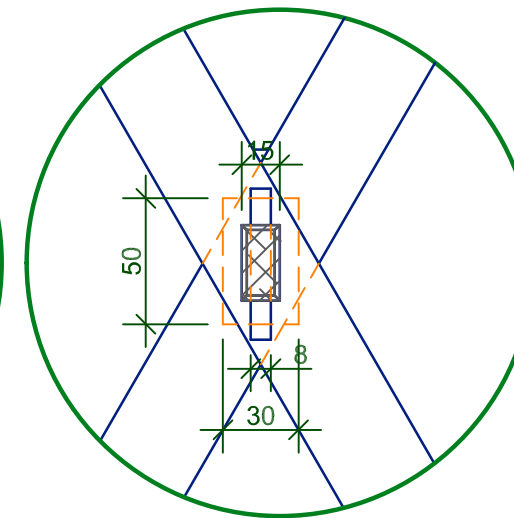
Detail 2 Scale 1:3
