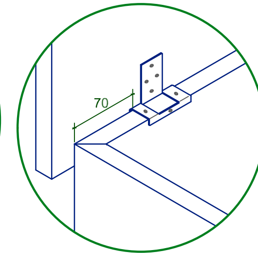
Hinge Placement Detail
