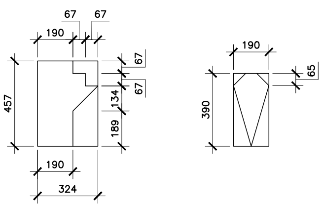
PLAN VIEW VUE ASSISE
